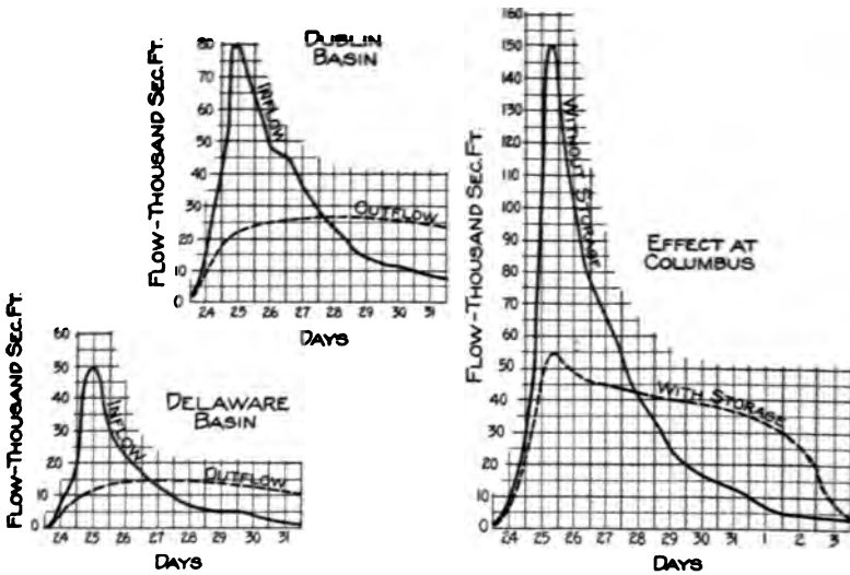
FIG. 41.—Diagram showing flow hydrographs for 150,000 sec. ft. flood with and without detention basins.
